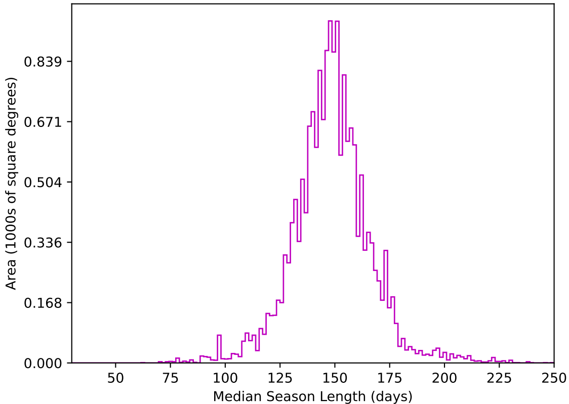
too_elab_r256_d2_gz_v3.4_10yrs WFD z band: Median Season Length
