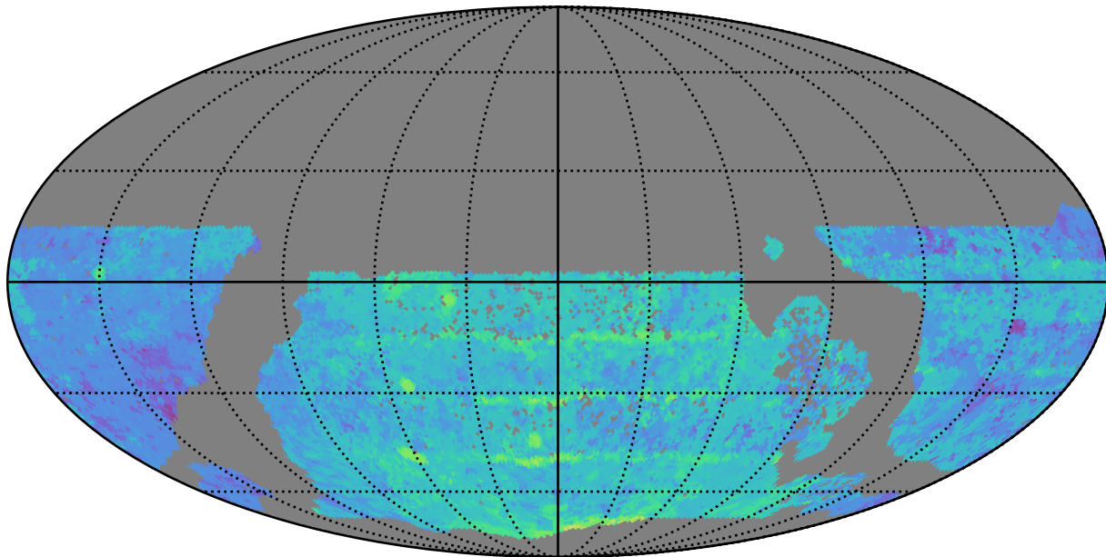
too_elab_r256_d2_gz_v3.4_10yrs WFD y band: Median Season Length
