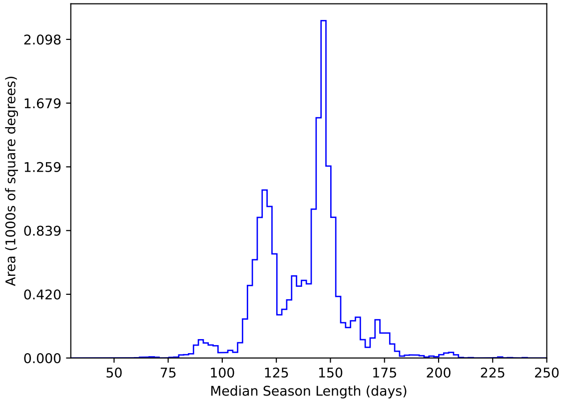
too_elab_r256_d2_gz_v3.4_10yrs WFD y band: Median Season Length
