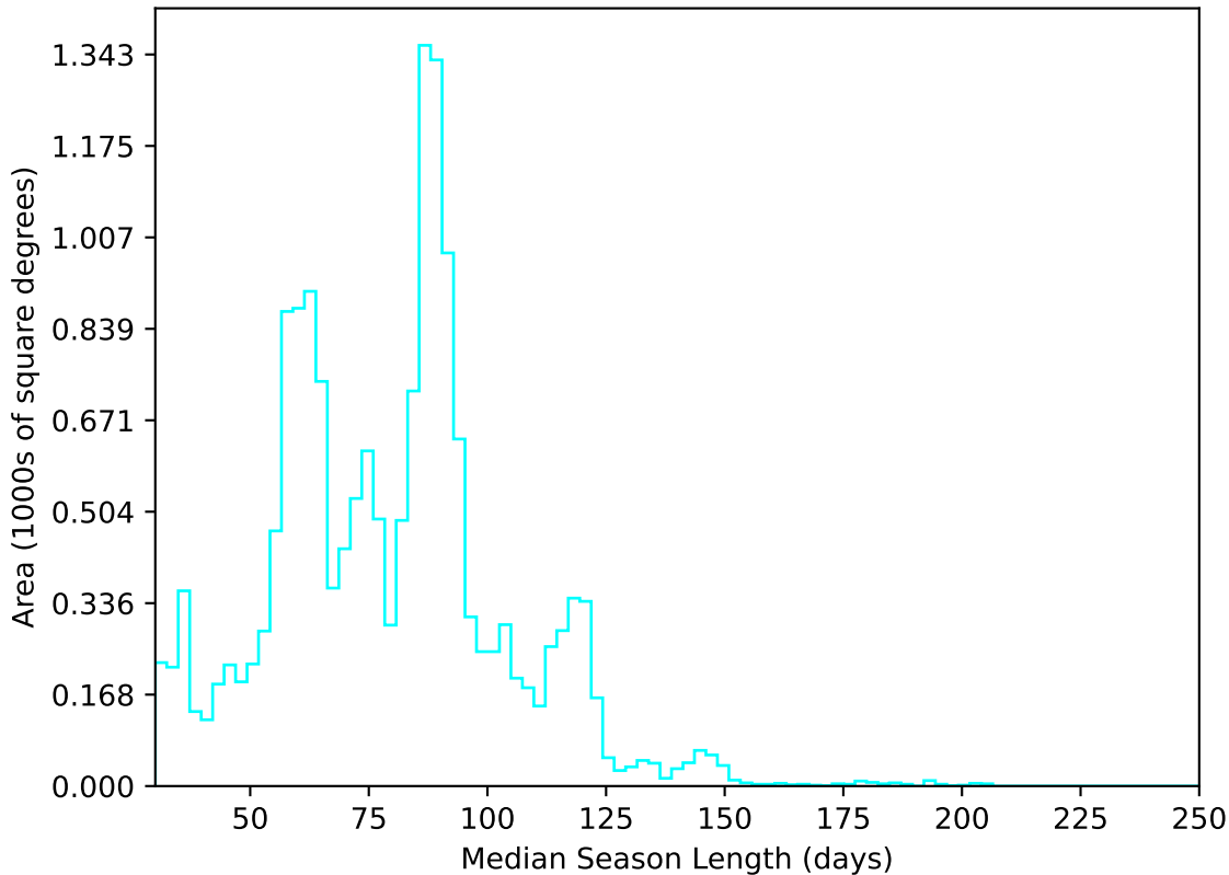
too_elab_r256_d2_gz_v3.4_10yrs WFD u band: Median Season Length
