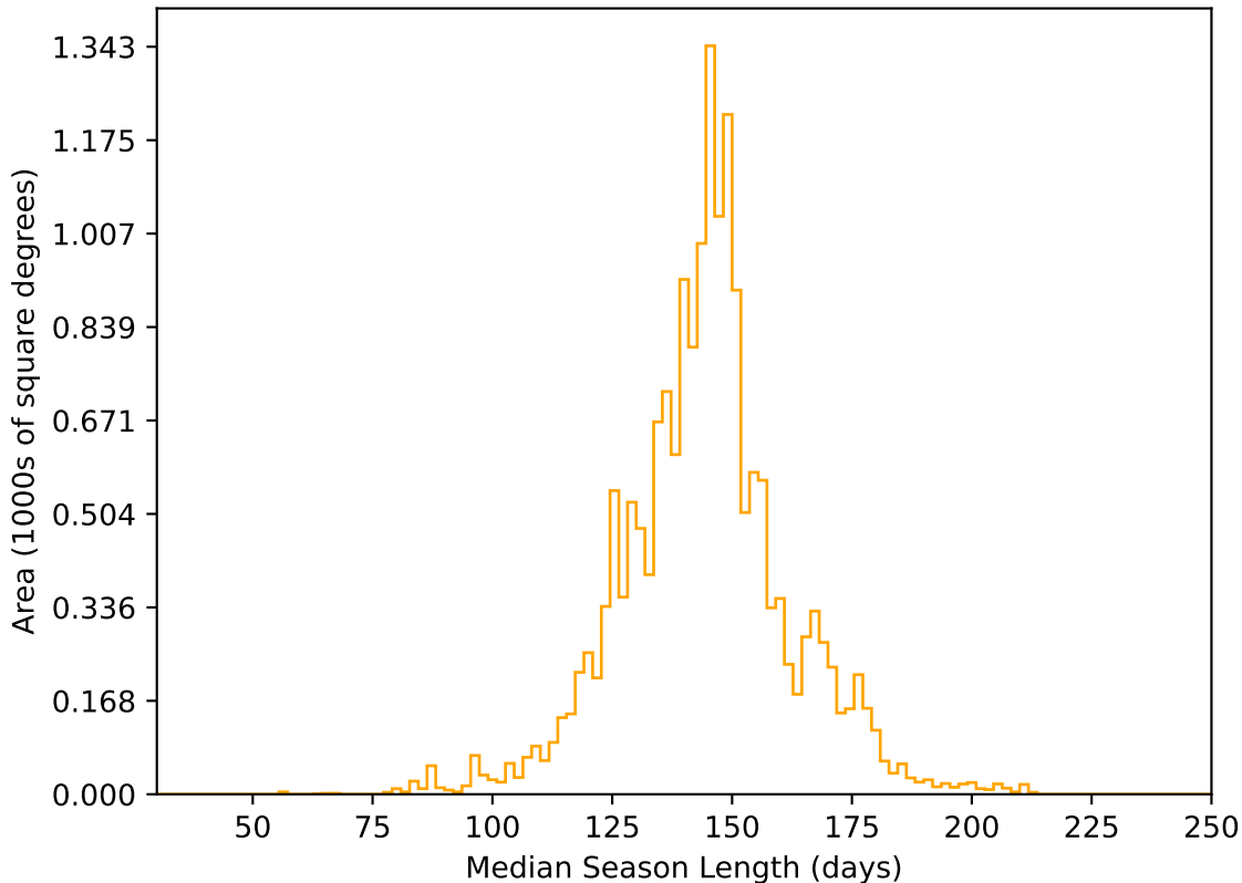
too_elab_r256_d2_gz_v3.4_10yrs WFD r band: Median Season Length
