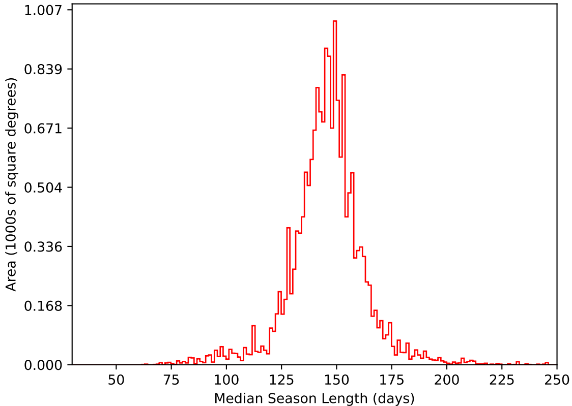
too_elab_r256_d2_gz_v3.4_10yrs WFD i band: Median Season Length
