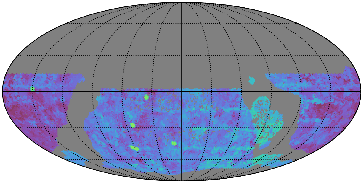
too_elab_r256_d2_gz_v3.4_10yrs WFD g band: Median Season Length
