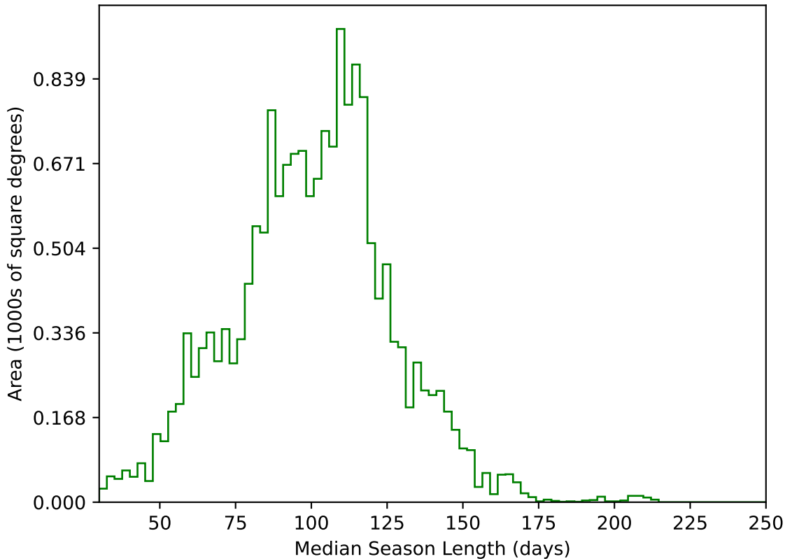
too_elab_r256_d2_gz_v3.4_10yrs WFD g band: Median Season Length
