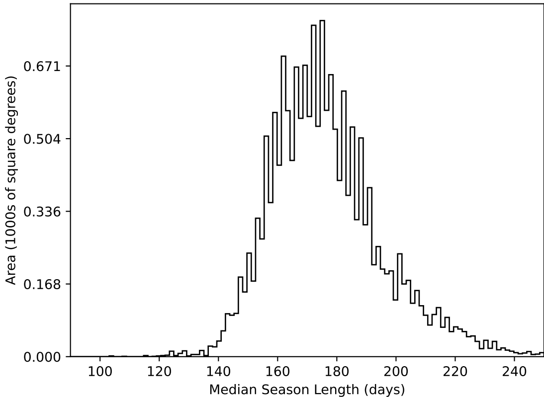
too_elab_r256_d2_gz_v3.4_10yrs WFD all bands: Median Season Length
