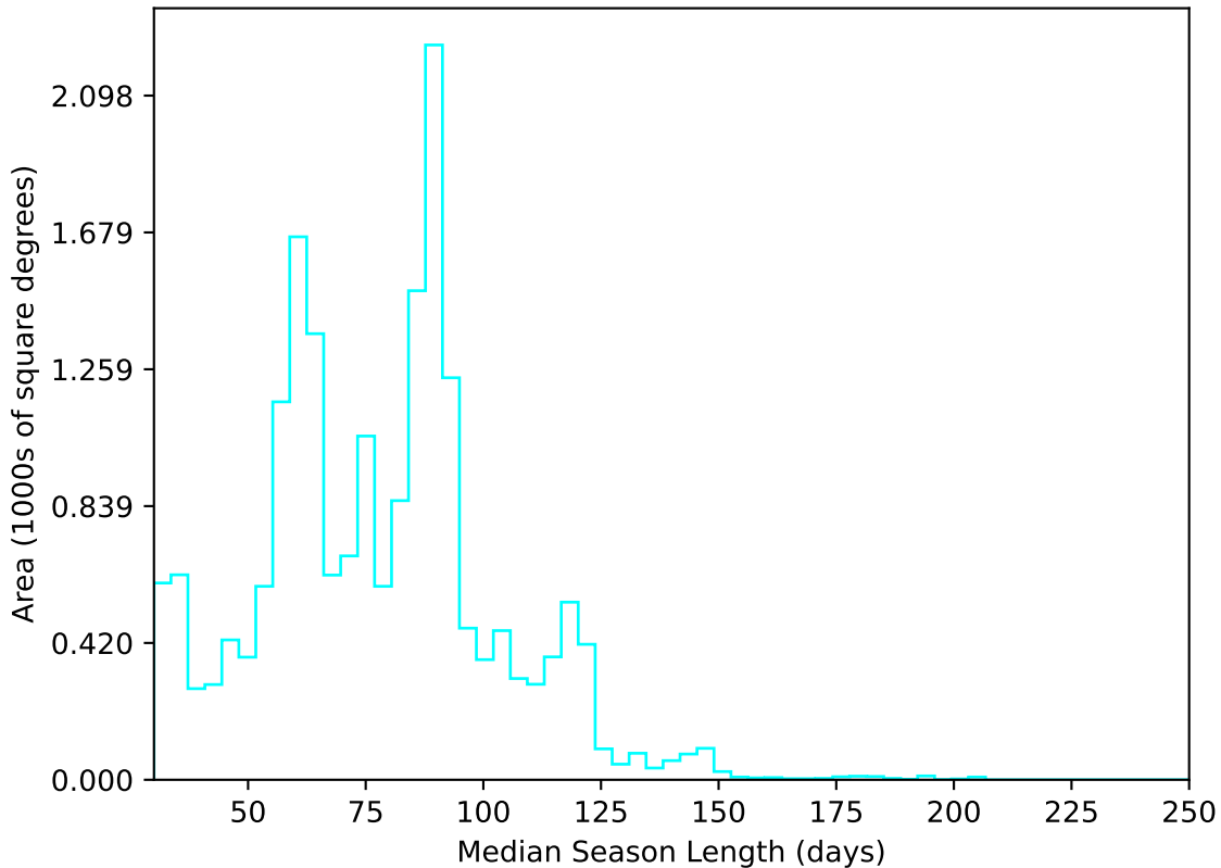
too_elab_r256_d2_gz_v3.4_10yrs All sky u band: Median Season Length
