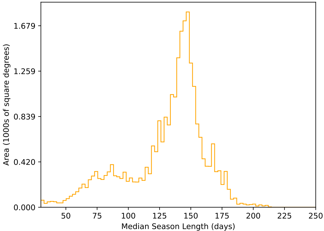
too_elab_r256_d2_gz_v3.4_10yrs All sky r band: Median Season Length
