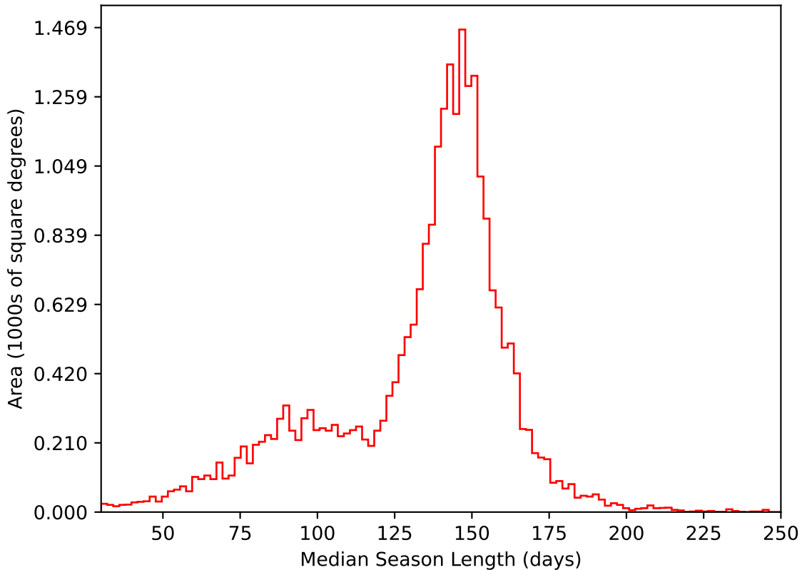
too_elab_r256_d2_gz_v3.4_10yrs All sky i band: Median Season Length
