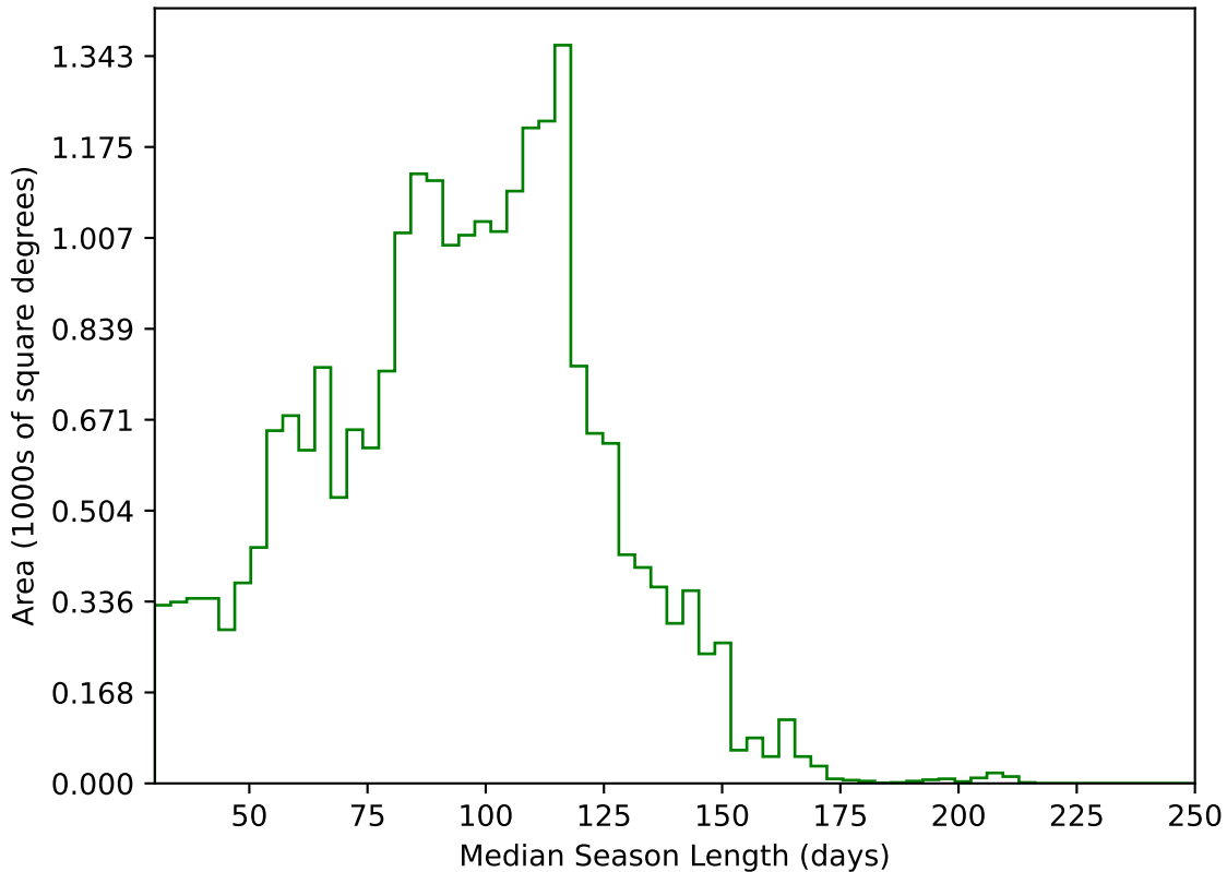
too_elab_r256_d2_gz_v3.4_10yrs All sky g band: Median Season Length
