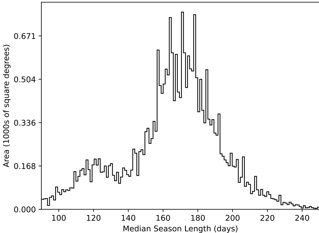
too_elab_r256_d2_gz_v3.4_10yrs All sky all bands: Median Season Length
