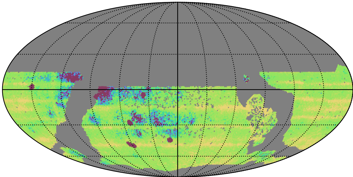
too_elab_r256_d2_gz_v3.4_10yrs WFD: Median Intra-Night Gap
