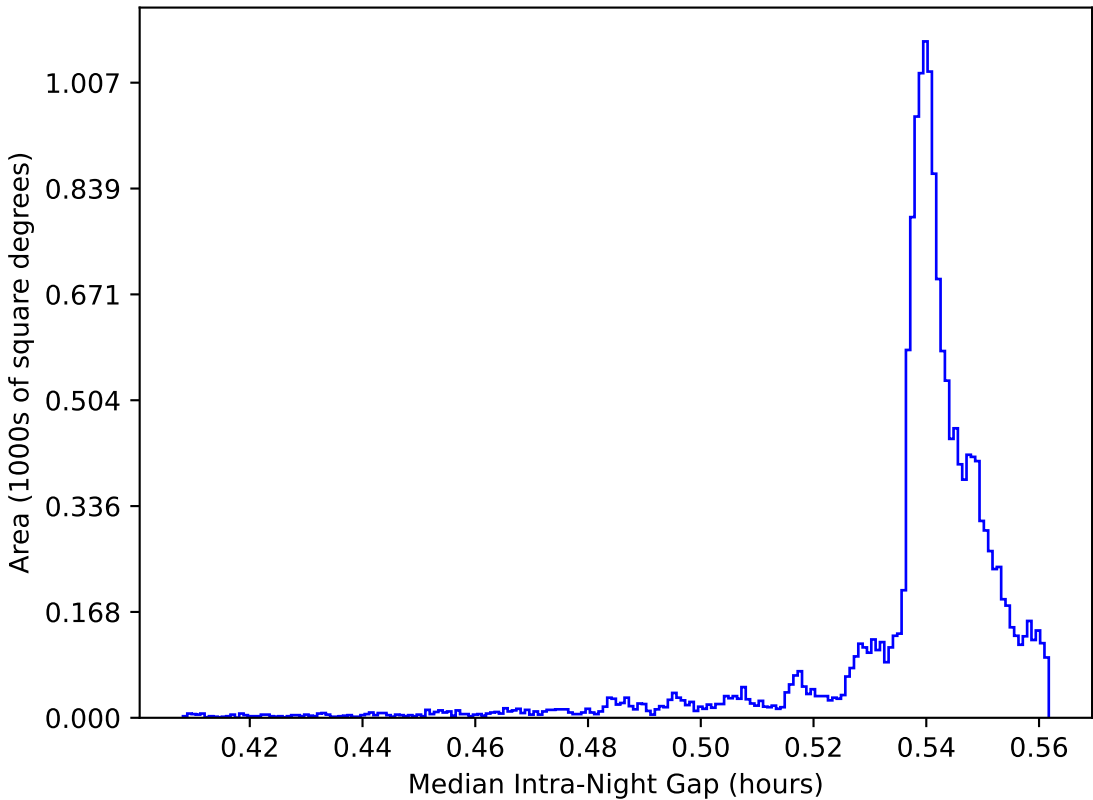
too_elab_r256_d2_gz_v3.4_10yrs WFD: Median Intra-Night Gap
