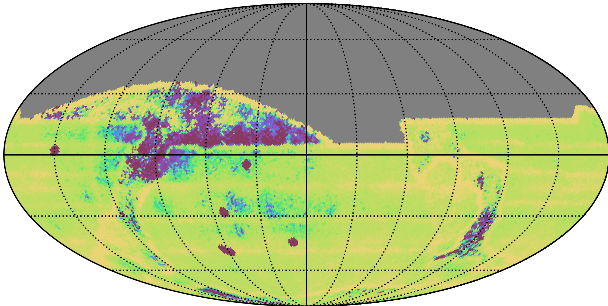
too_elab_r256_d2_gz_v3.4_10yrs All sky: Median Intra-Night Gap
