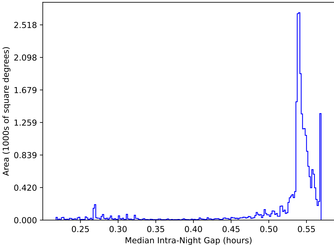
too_elab_r256_d2_gz_v3.4_10yrs All sky: Median Intra-Night Gap
