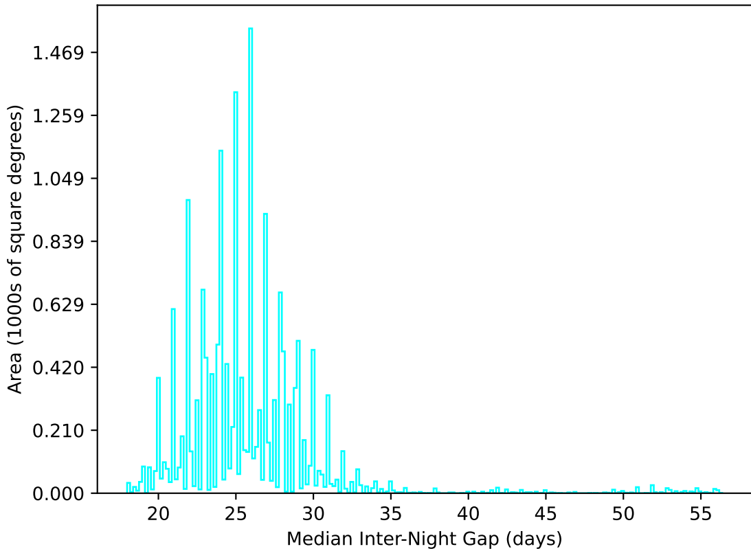
too_elab_r256_d2_gz_v3.4_10yrs WFD u band: Median Inter-Night Gap
