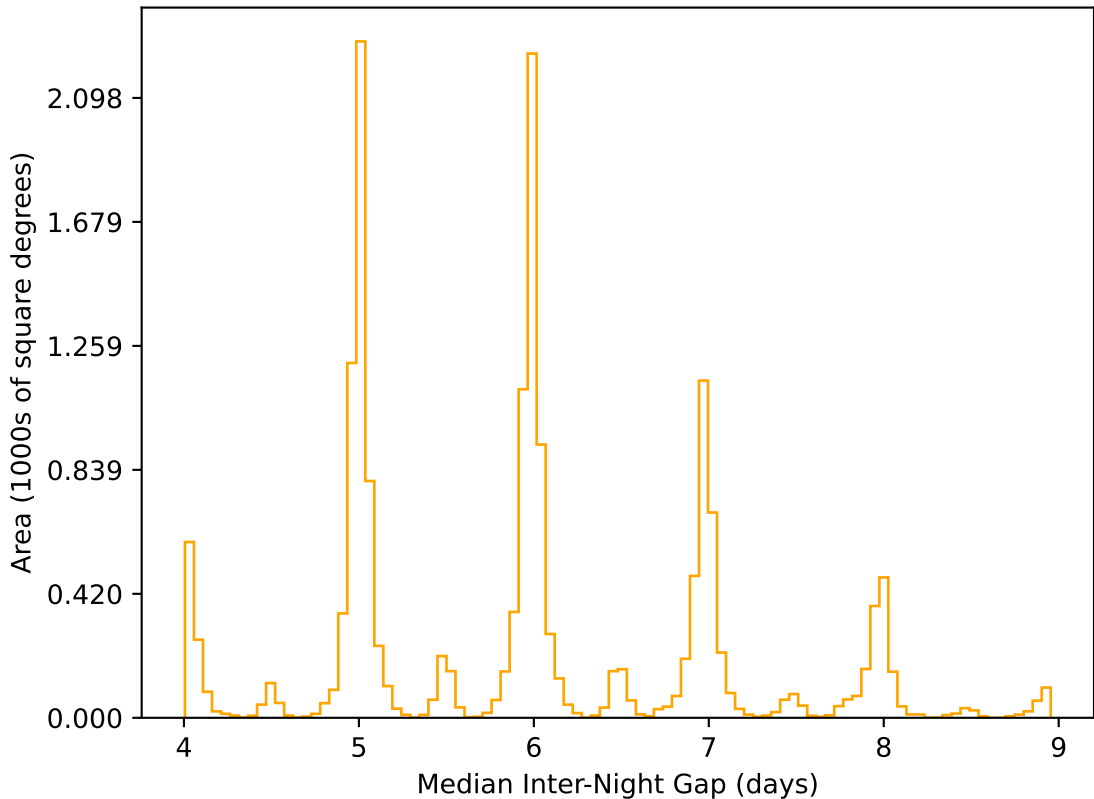
too_elab_r256_d2_gz_v3.4_10yrs WFD r band: Median Inter-Night Gap
