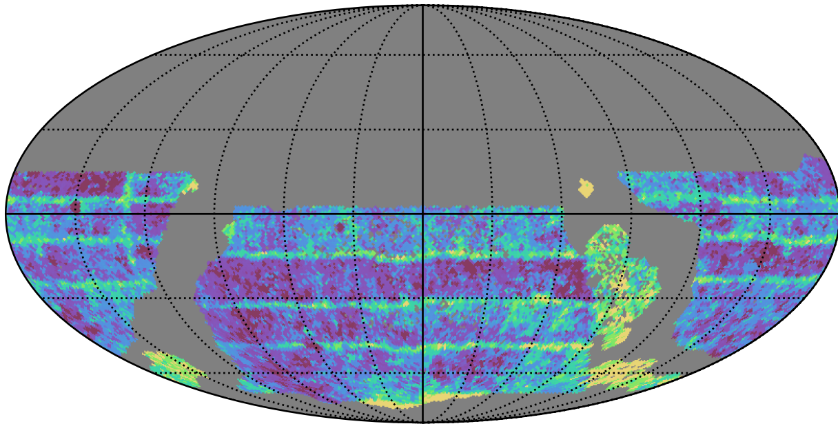
too_elab_r256_d2_gz_v3.4_10yrs WFD i band: Median Inter-Night Gap
