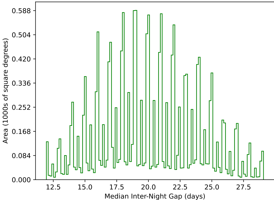
too_elab_r256_d2_gz_v3.4_10yrs WFD g band: Median Inter-Night Gap
