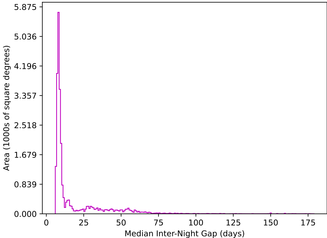
too_elab_r256_d2_gz_v3.4_10yrs All sky z band: Median Inter-Night Gap
