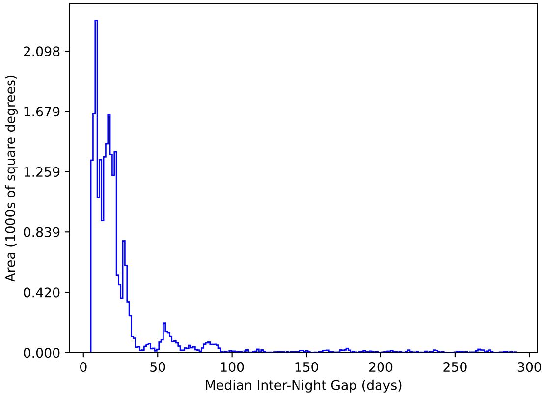
too_elab_r256_d2_gz_v3.4_10yrs All sky y band: Median Inter-Night Gap
