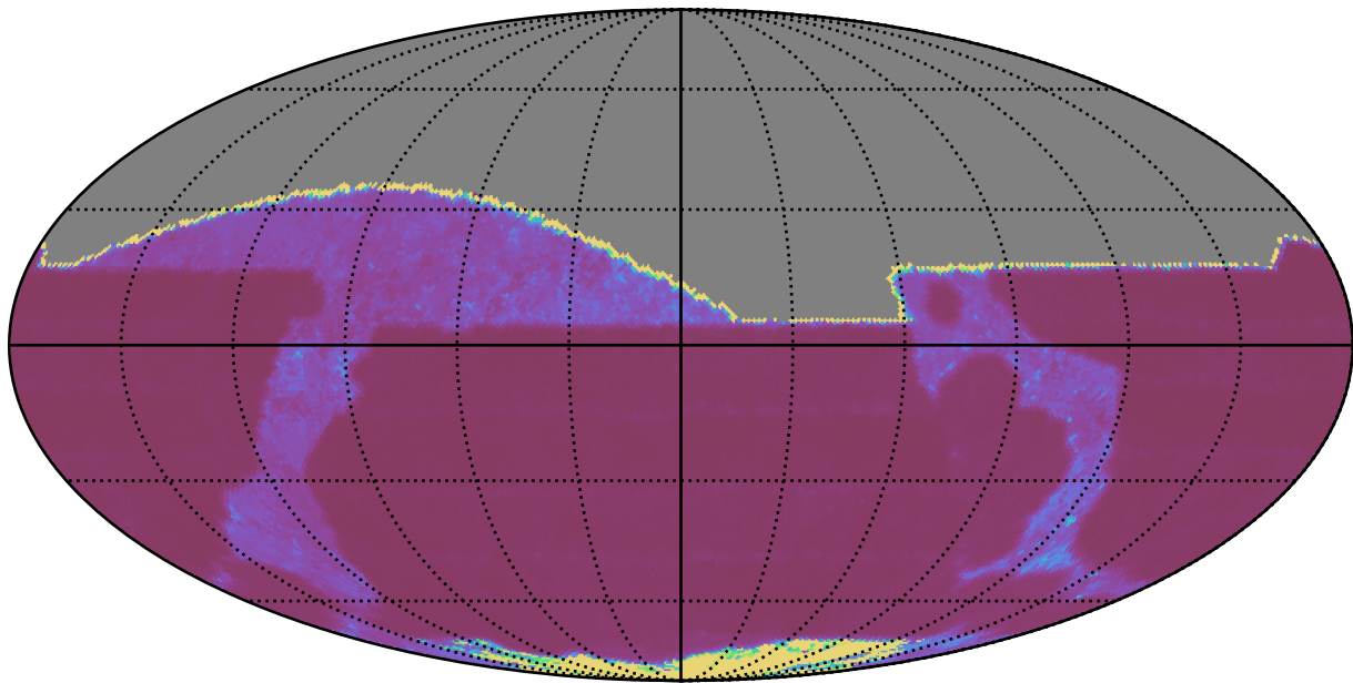
too_elab_r256_d2_gz_v3.4_10yrs All sky r band: Median Inter-Night Gap
