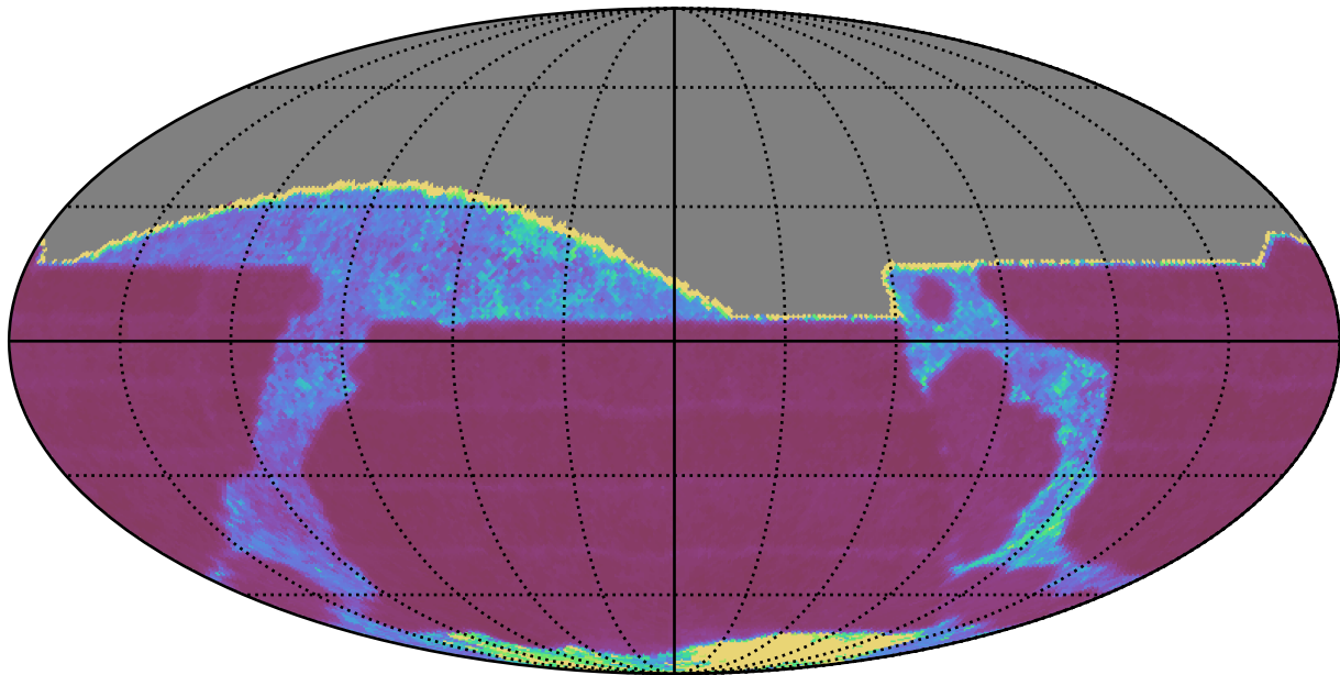
too_elab_r256_d2_gz_v3.4_10yrs All sky i band: Median Inter-Night Gap
