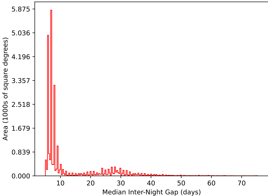
too_elab_r256_d2_gz_v3.4_10yrs All sky i band: Median Inter-Night Gap
