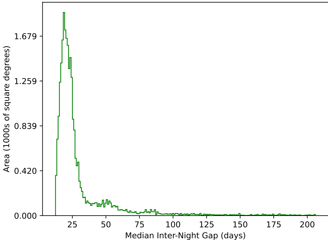
too_elab_r256_d2_gz_v3.4_10yrs All sky g band: Median Inter-Night Gap
