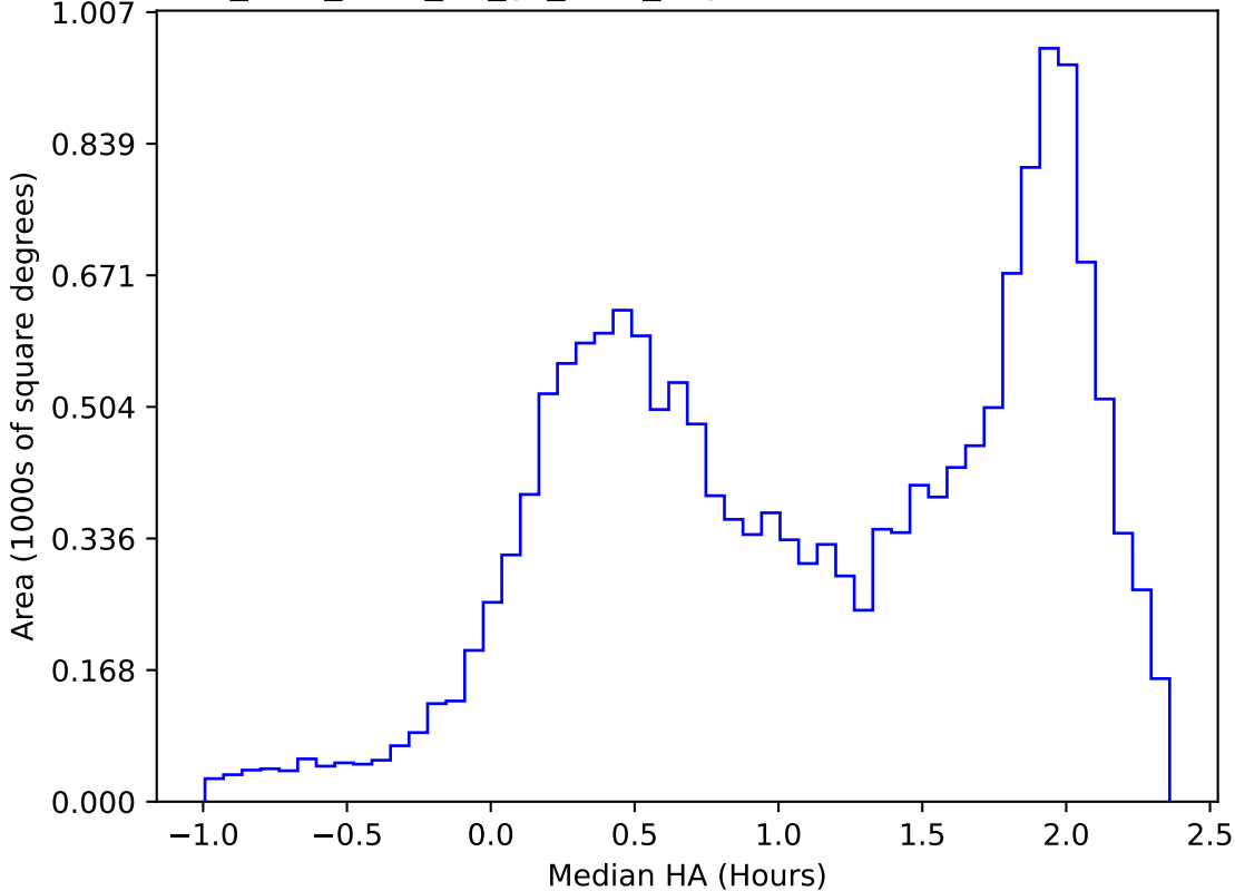
too_elab_r256_d2_gz_v3.4_10yrs WFD z band: Median HA
