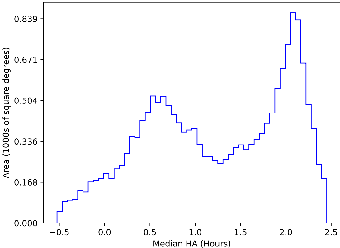
too_elab_r256_d2_gz_v3.4_10yrs WFD y band: Median HA
