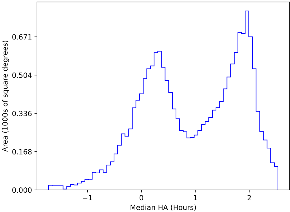
too_elab_r256_d2_gz_v3.4_10yrs WFD u band: Median HA
