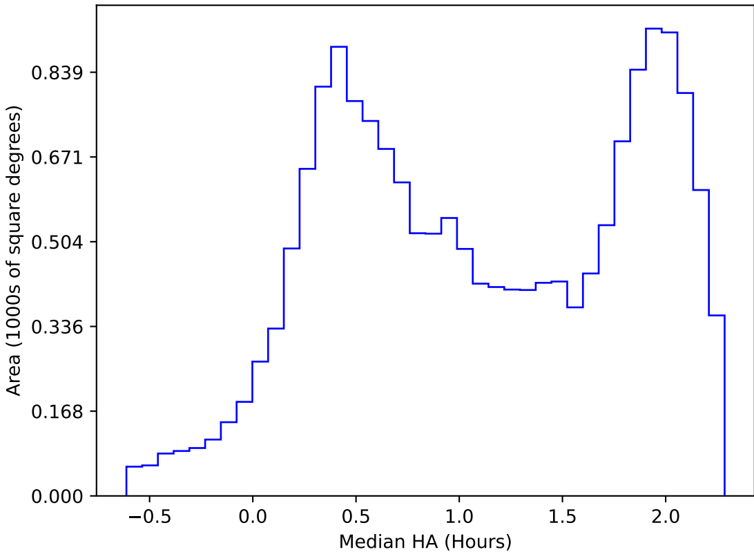
too_elab_r256_d2_gz_v3.4_10yrs WFD i band: Median HA
