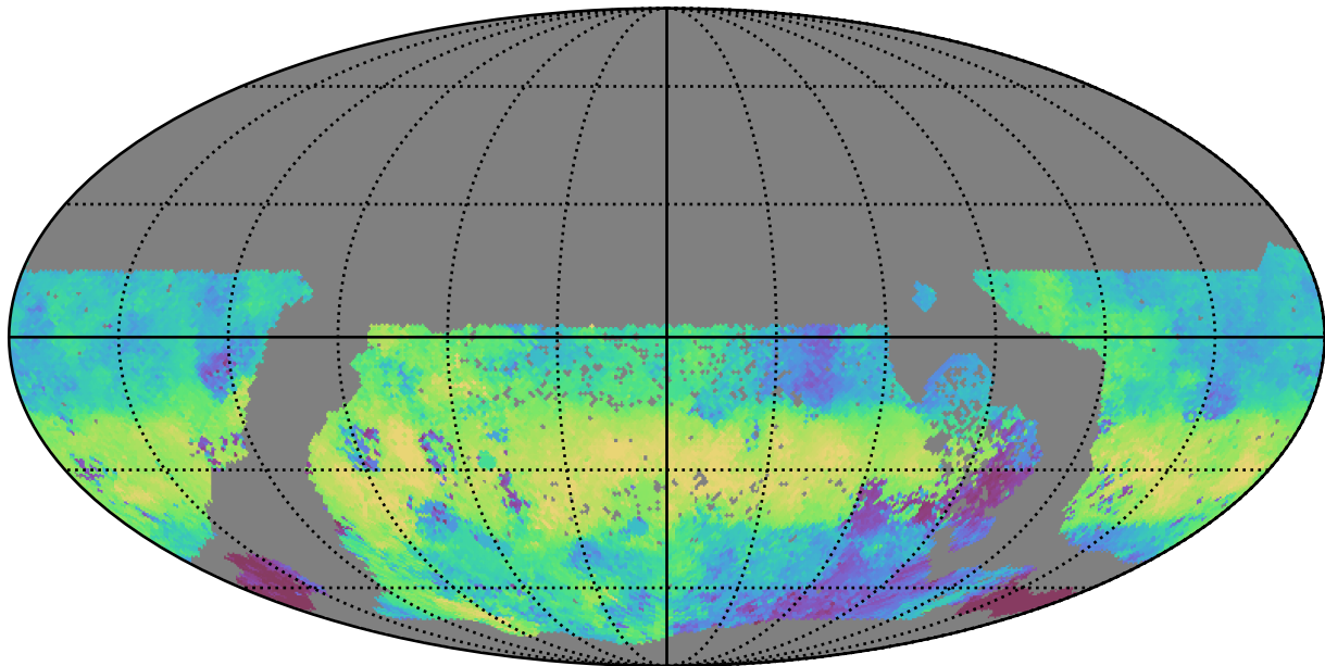
too_elab_r256_d2_gz_v3.4_10yrs WFD g band: Median HA
