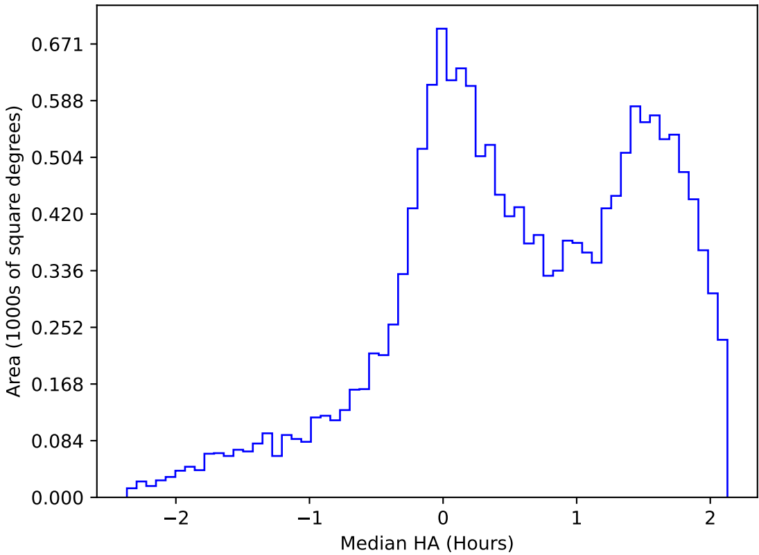
too_elab_r256_d2_gz_v3.4_10yrs WFD g band: Median HA
