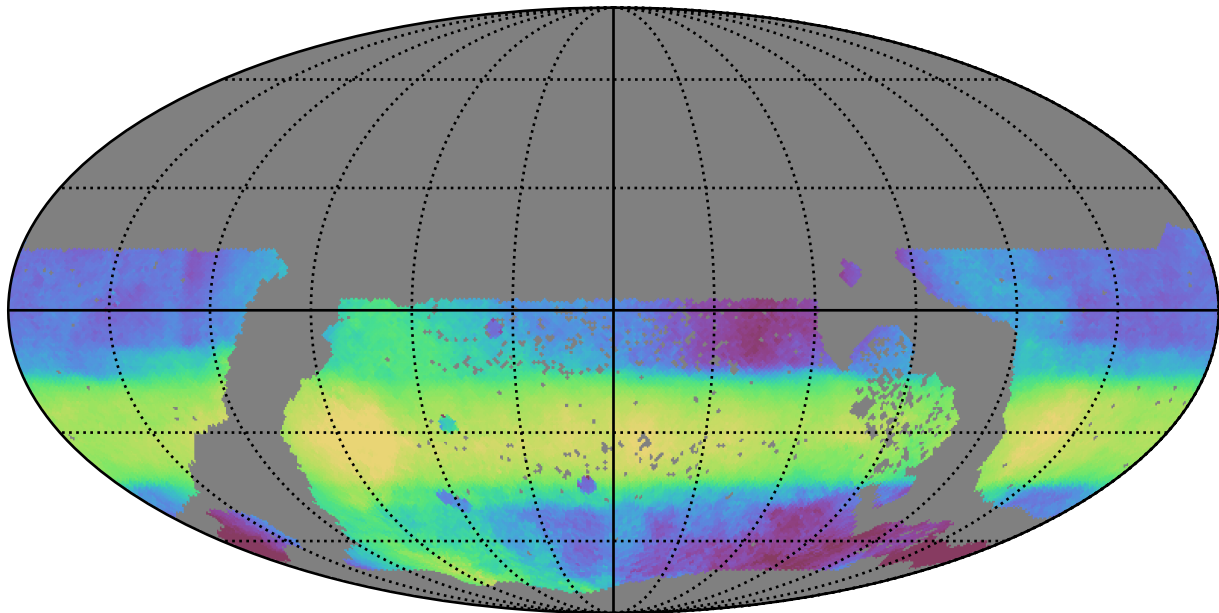
too_elab_r256_d2_gz_v3.4_10yrs WFD all bands: Median HA
