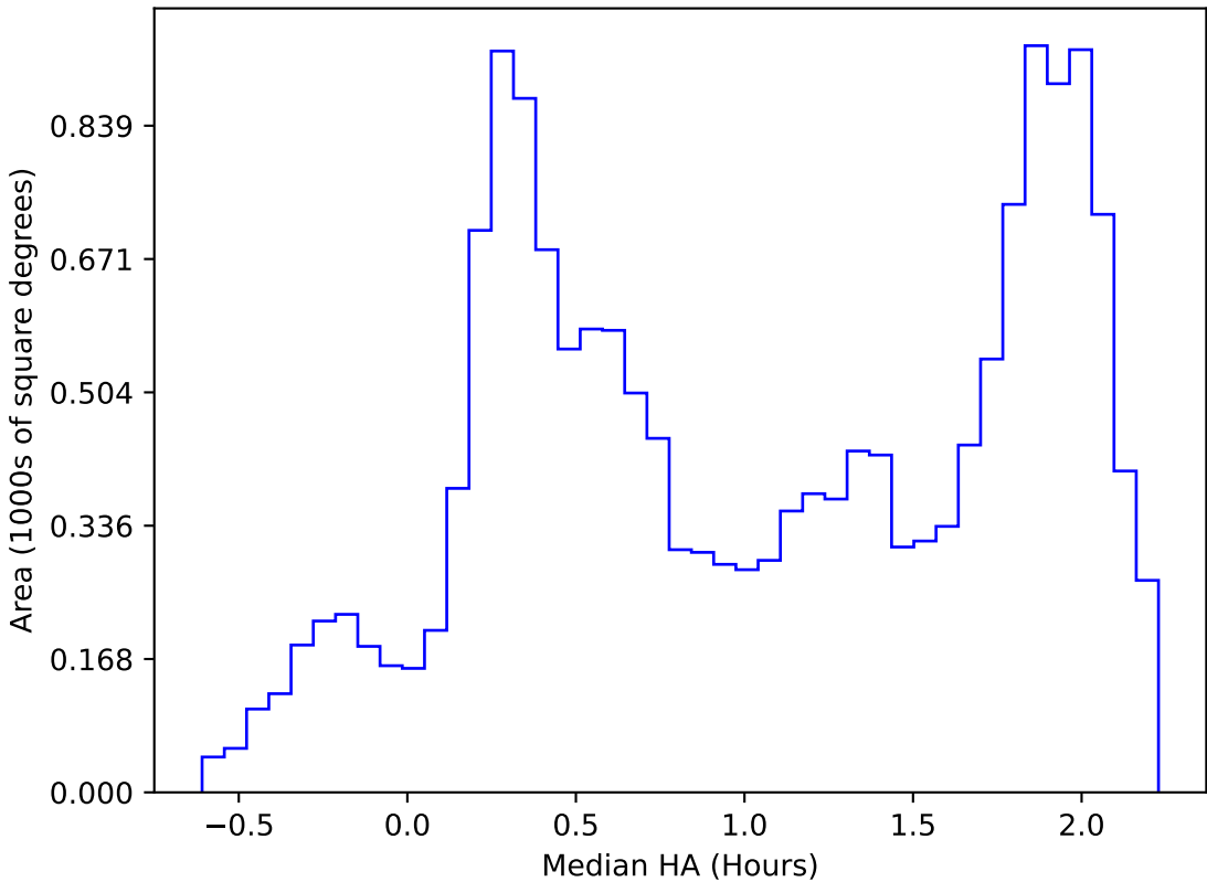
too_elab_r256_d2_gz_v3.4_10yrs WFD all bands: Median HA
