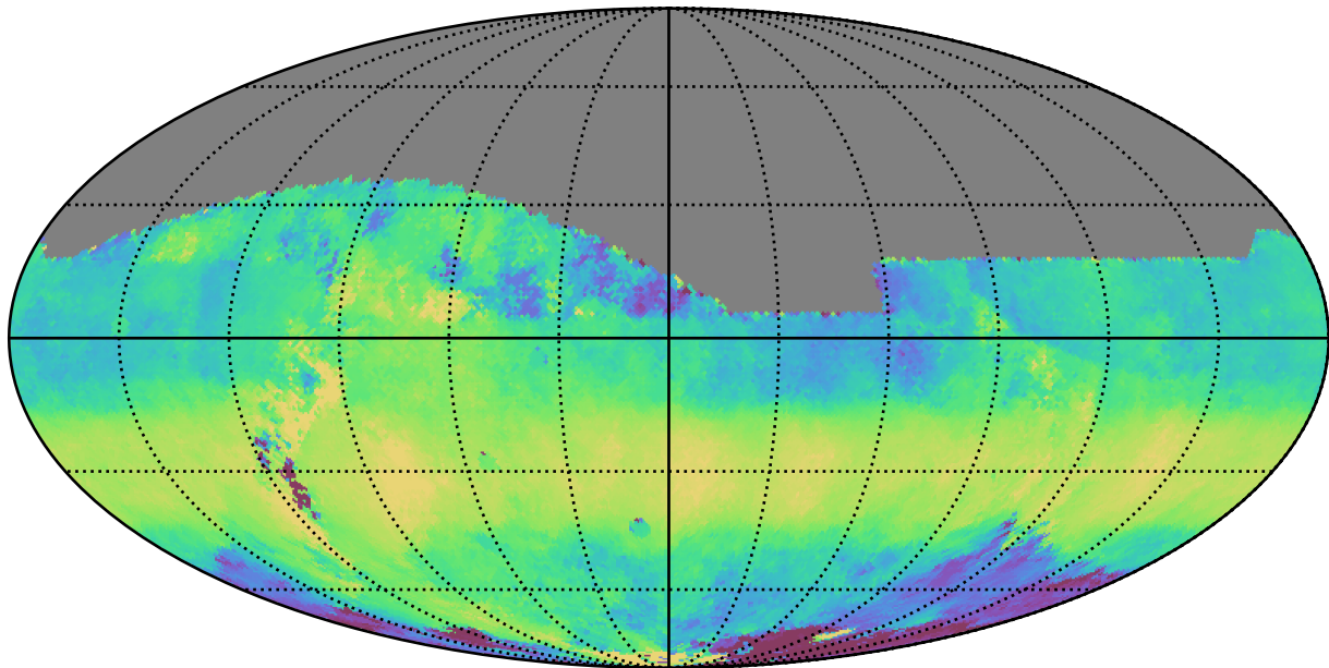
too_elab_r256_d2_gz_v3.4_10yrs All sky z band: Median HA
