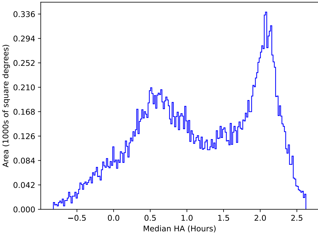
too_elab_r256_d2_gz_v3.4_10yrs All sky y band: Median HA
