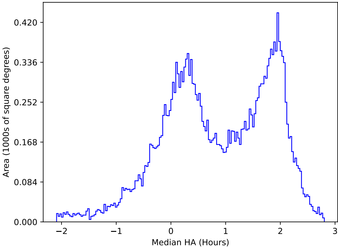
too_elab_r256_d2_gz_v3.4_10yrs All sky u band: Median HA
