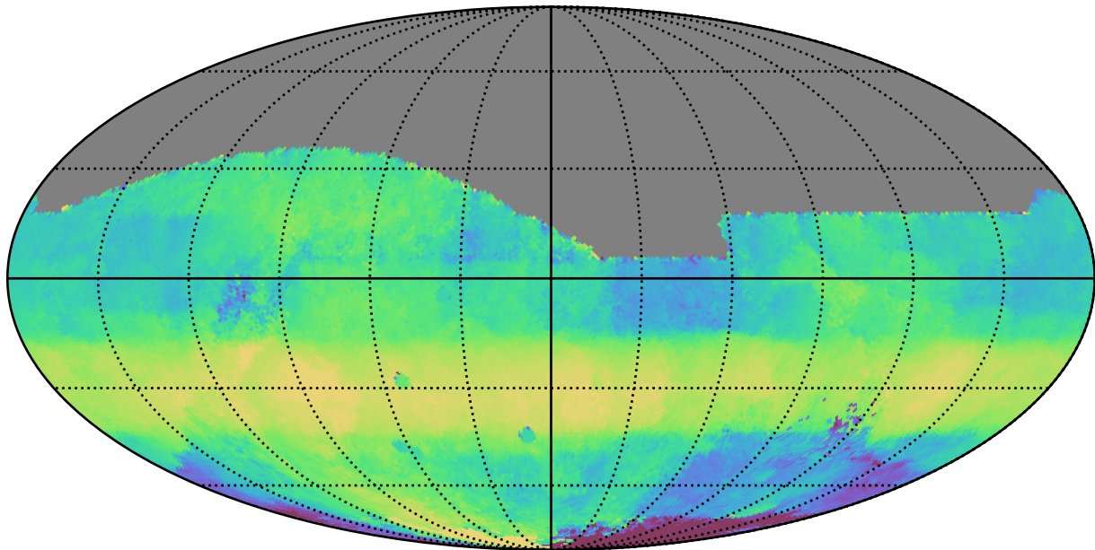
too_elab_r256_d2_gz_v3.4_10yrs All sky r band: Median HA
