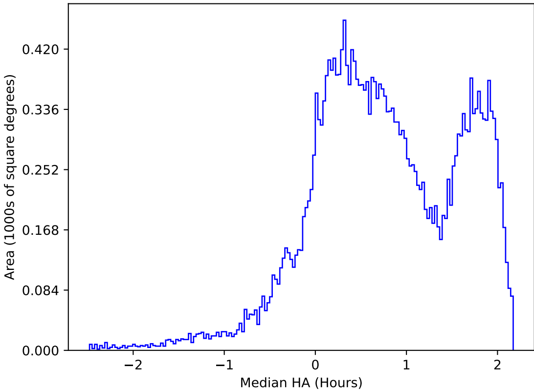
too_elab_r256_d2_gz_v3.4_10yrs All sky r band: Median HA
