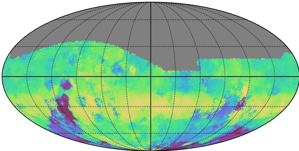
too_elab_r256_d2_gz_v3.4_10yrs All sky g band: Median HA
