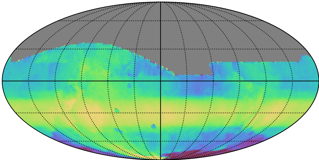
too_elab_r256_d2_gz_v3.4_10yrs All sky all bands: Median HA
