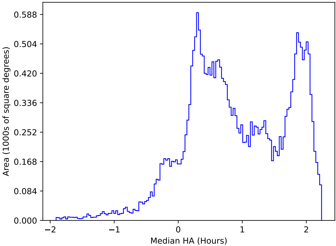
too_elab_r256_d2_gz_v3.4_10yrs All sky all bands: Median HA
