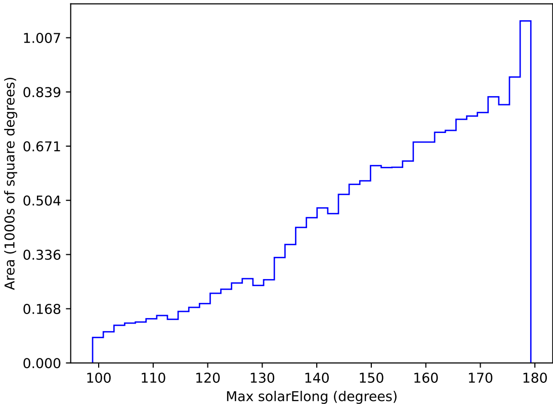
too_elab_r256_d2_gz_v3.4_10yrs WFD z band: Max solarElong
