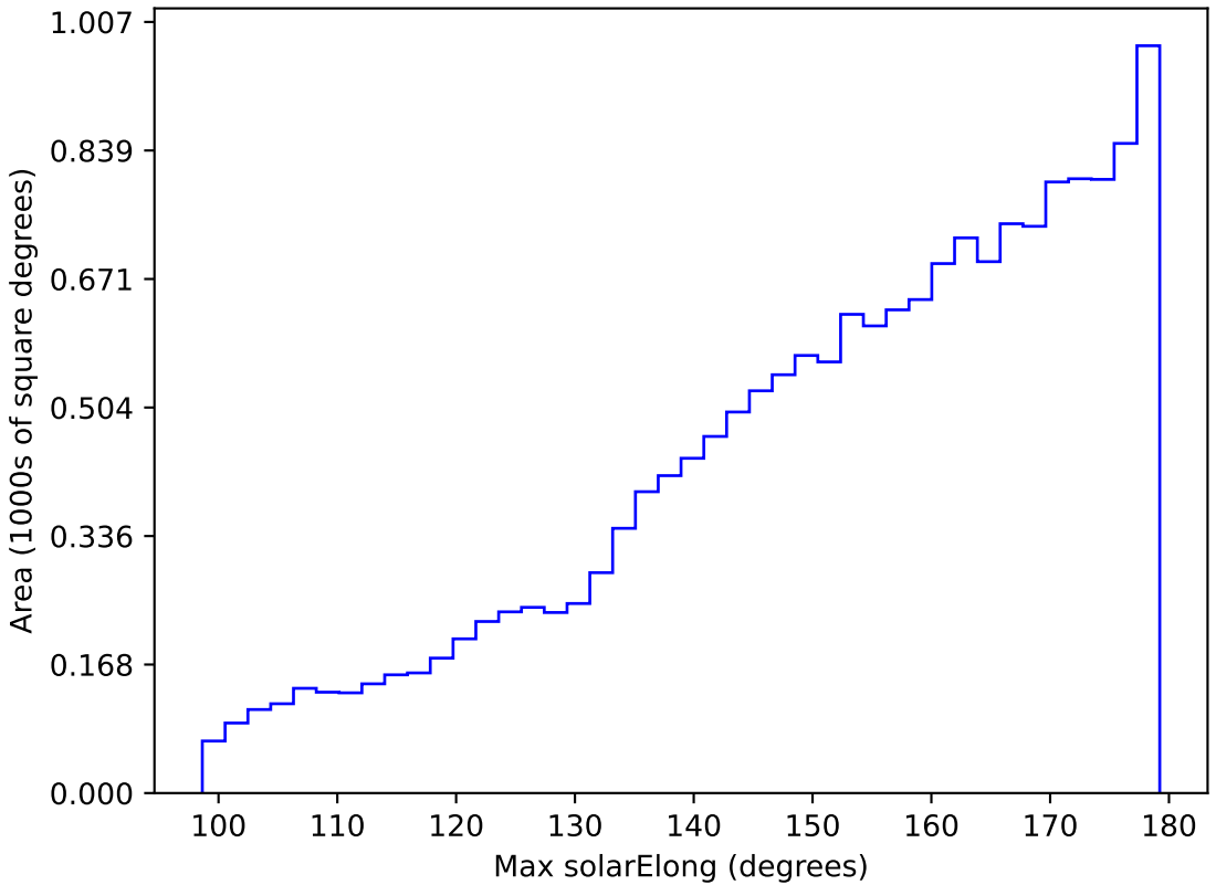
too_elab_r256_d2_gz_v3.4_10yrs WFD y band: Max solarElong
