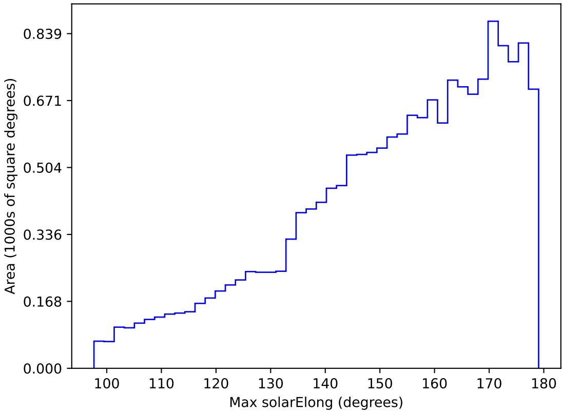
too_elab_r256_d2_gz_v3.4_10yrs WFD u band: Max solarElong
