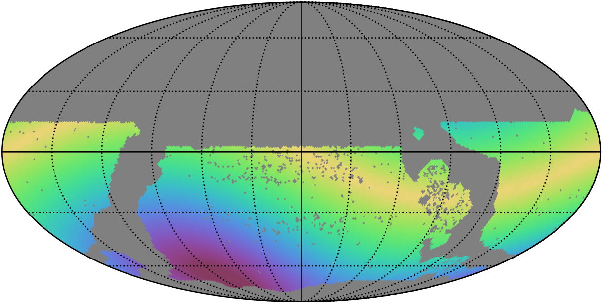
too_elab_r256_d2_gz_v3.4_10yrs WFD r band: Max solarElong
