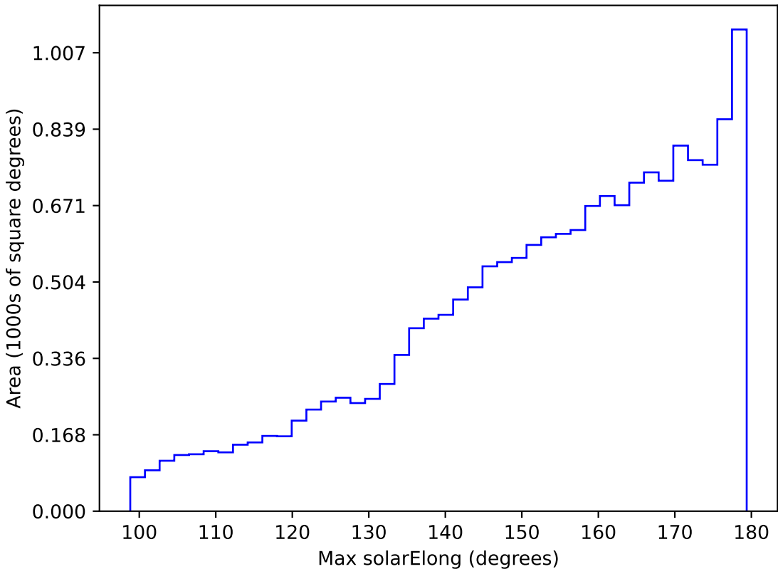
too_elab_r256_d2_gz_v3.4_10yrs WFD r band: Max solarElong
