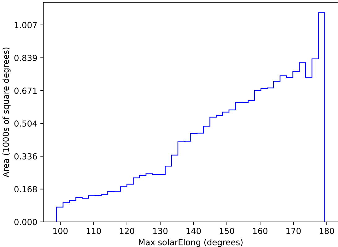
too_elab_r256_d2_gz_v3.4_10yrs WFD i band: Max solarElong
